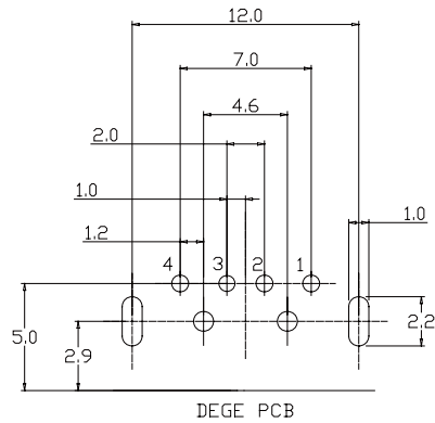
DEGE PCB
